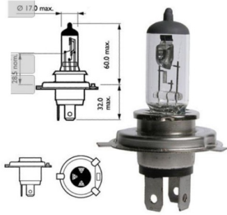
H 4 Bulb With Pin
