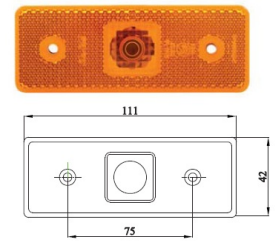
0304 Side Marker Lamp
